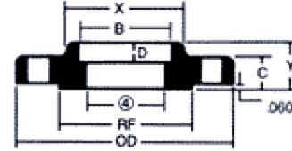
SOCKET WELD
