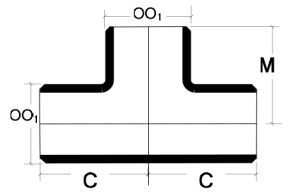
Straight Tee
