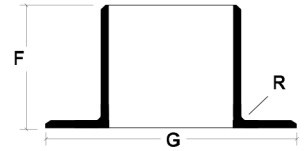
Short Pattern Stub End
