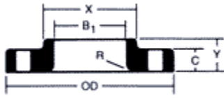
LAP JOINT
