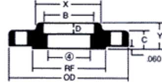
SOCKET WELD
