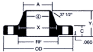
WELD NECK
