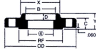
SOCKET WELD
