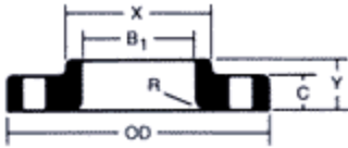
LAP JOINT
